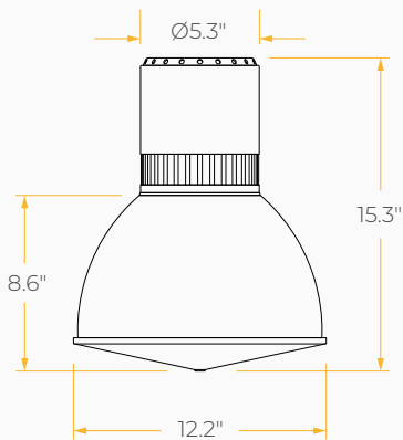
Conical Lens 12"
