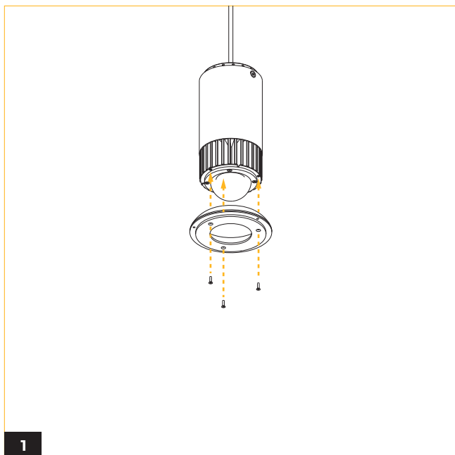
1 Fasten Shroud Mounting plate using three phillips screws.
