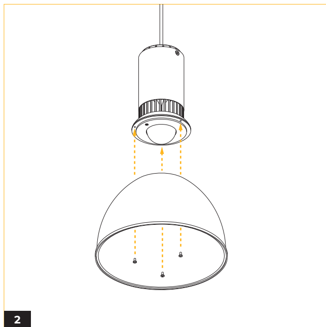
2 Bring shroud to the fixture level and align it to the indicated openings. Fasten shroud in place with three phillips screws.
