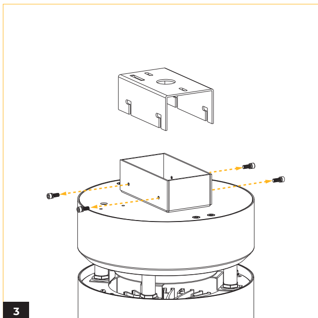
3 Loosen the screws that secure the mounting brackets and detach the upper mounting bracket and safety hook.
