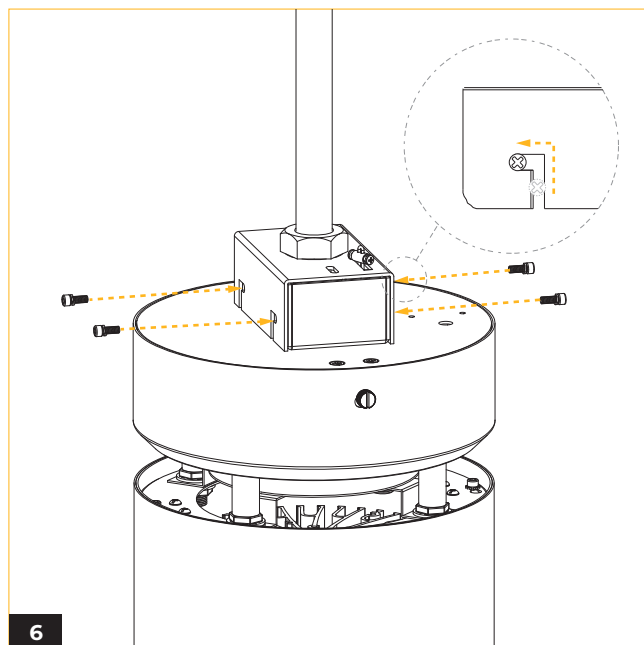
6 Fasten the 2 screw nuts on either side of the mounting bracket including the safety cable.
