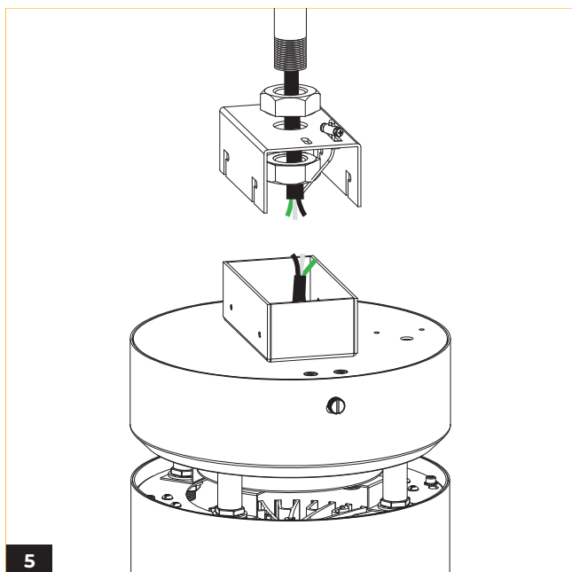
5 Loop and fasten the safety cable through the slot available on the mounting bracket.
