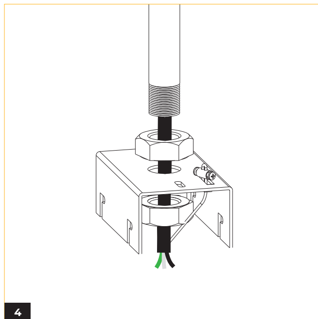
4 Insert Wire cable and safety cable through the 2 screw nuts placed on either side of the mounting bracket.
