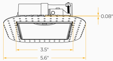
Round Flangeless Trim
