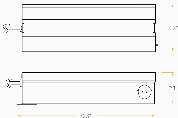
Retrofit Power Box (DMXP/DMXR)
