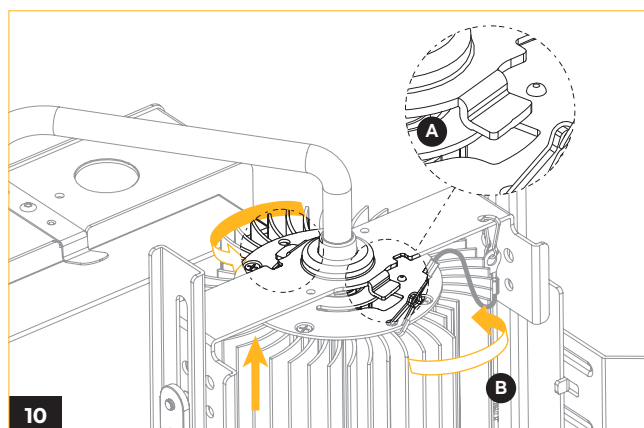
Adjust the light engine into the support and slightly turn it to the right to secure it.
