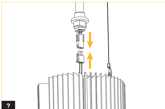
Connect the electrical connections.
