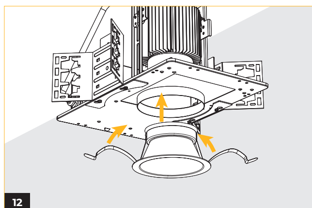
Insert the trim through the hole with the springs bent inwardly.
