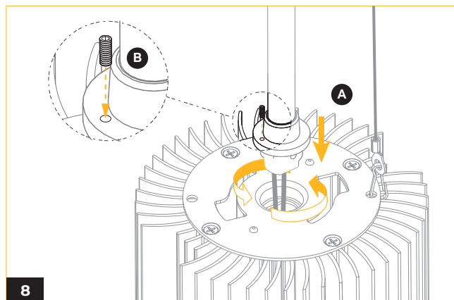
Connect the conduit to the light engine and slightly turn it to the right to secure it. Tighten the socket set screw to secure the conduit.
