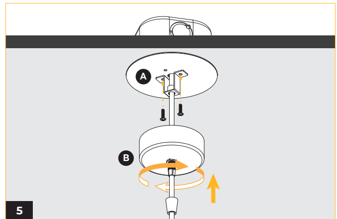
(A) Fasten canopy plate in place using 2 phillips screws.
