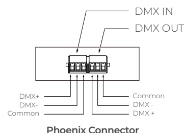
Phoenix Connector
