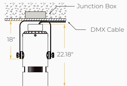
Yoke Mount
