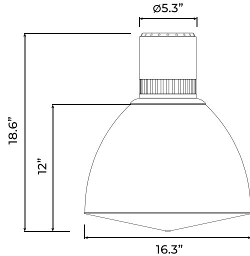
Conical Lens 16"
