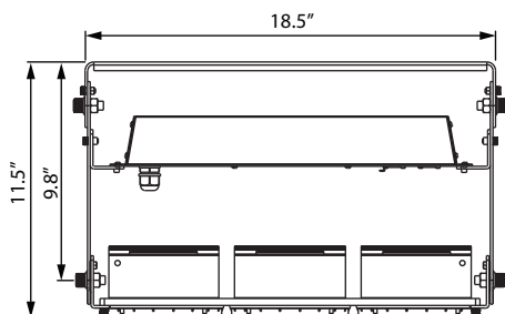
Bracket Mount / 3 Modules
