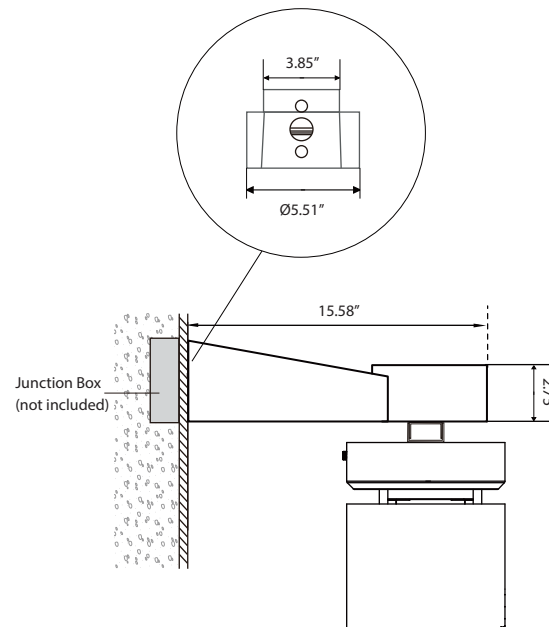
Wall Mount
