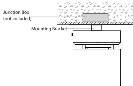
Surface Mount
