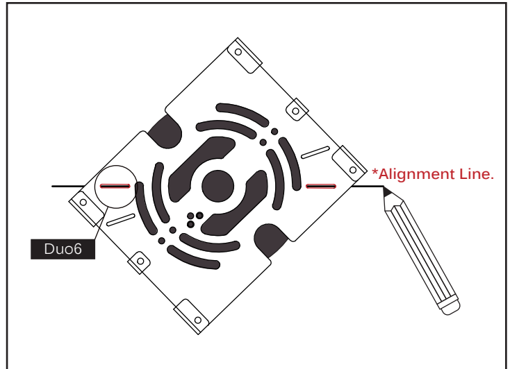
Step 7 Mark an alignment line on the ceiling and align it with the indicated markers on the mounting plate. The mounting plate will be slanted at an angle in relation to the horizontal line as shown in the diagram.
