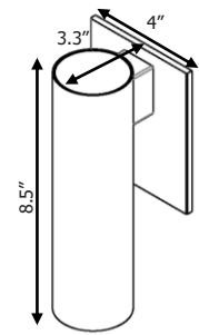
Wall Mount
