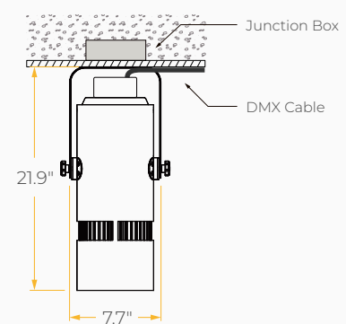
Yoke Mount
