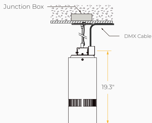
Adjustable Cable
