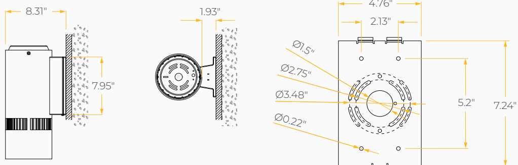
Wall Mount
