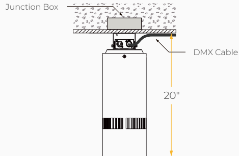
Surface Mount
