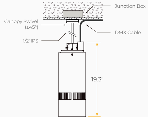
Stem Mount
