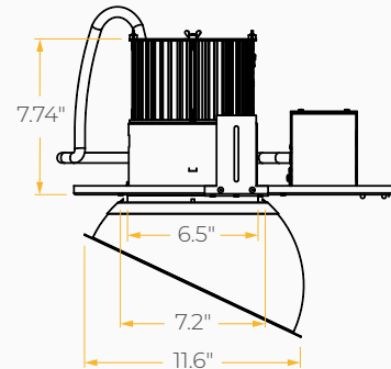
Sloped Ceiling Adapter
