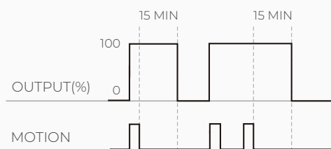
Occupancy Sensor Operation
