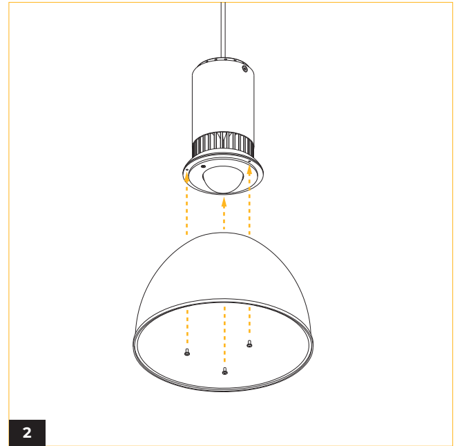
Bring shroud to the fixture level and align it to the indicated openings. Fasten shroud in place with three phillips screws.
