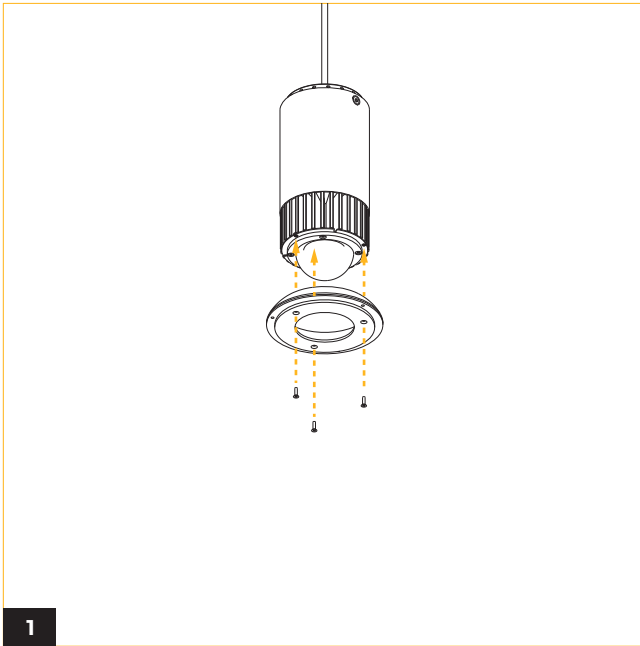
Fasten Shroud Mounting plate using three phillips screws.
