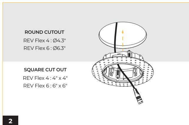
2 Insert the frame through the ceiling cut out.
