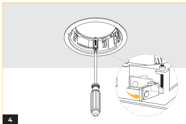
4 Use a Phillips screwdriver to expand the two mounting tabs and secure the bezel frame in place.
