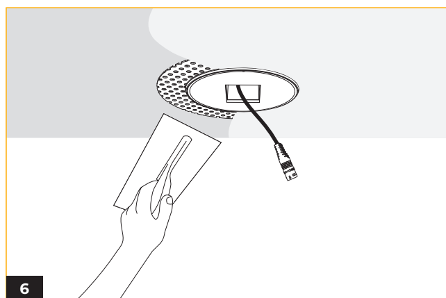
6 Spread the plastering compound evenly around the frame and smooth it out to create a flat surface on the ceiling. Once finished, remove the protective foam and proceed with the rest of the installation.
