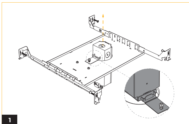
1 Align the extruded power box clip with the clasp insert on the new construction frame. Push up and hold in place.
