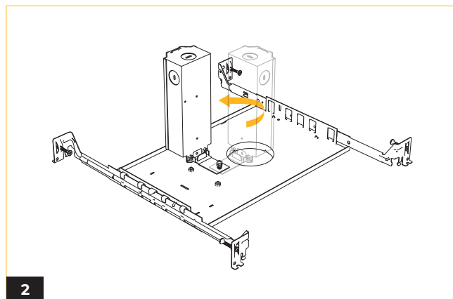
2 Push the power box aside along the alignment tracks to secure the power box and make room for the light engine.
