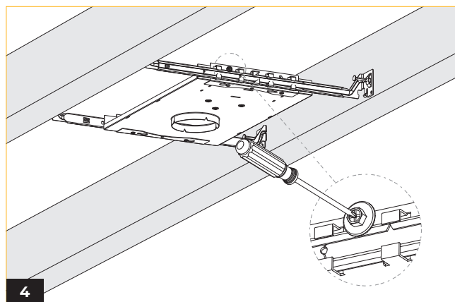
4 After securing the screw/nails in place, tighten the screws on the support rails to lock them from moving.
