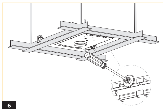
6 After securing the support rails in place, tighten the screws on the support rails to lock them from moving.
