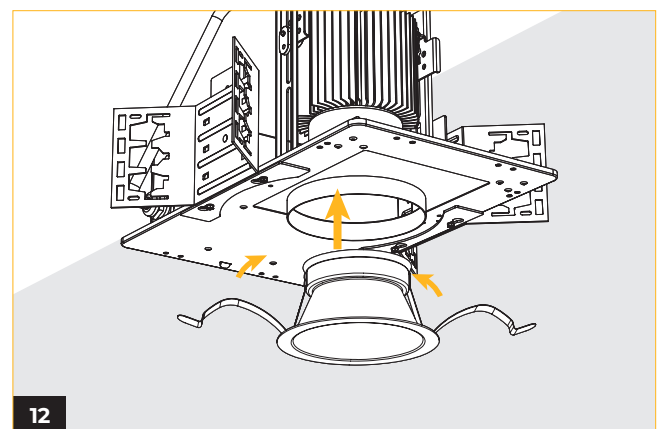
12 Insert the trim through the hole with the springs bent inwardly.
