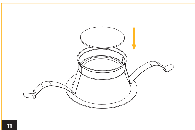
11 Attach the diffuser to the trim.
