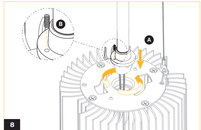
8 Connect the conduit to the light engine and slightly turn it to the right to secure it. Tighten the socket set screw to secure the conduit.
