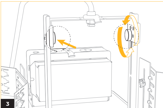
3 Loosen the knob on the bracket to adjust height according to the ordered trim.
