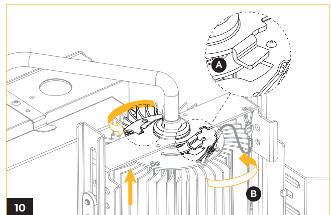
10 Adjust the light engine into the support and slightly turn it to the right to secure it.
