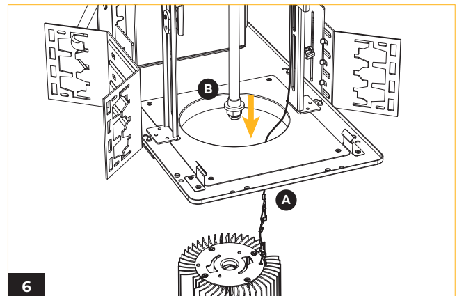
6 Connect the safety cables of both the bracket and the light engine, and pull the conduit to the outside.
