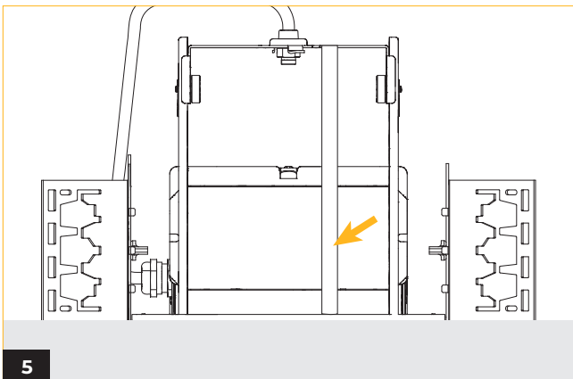
5 Adjust the bracket's height according to the L-tool starting from the outer part of the surface. Use the L-tool on each side to make sure both sides are balanced. Secure the knobs on the bracket once the height is adjusted.
