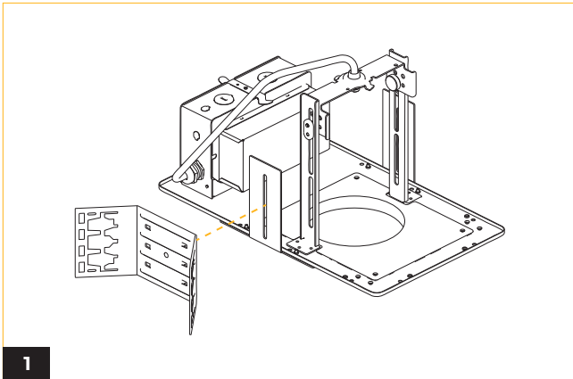
1 Align and attach the butterfly bracket to the side rail.
