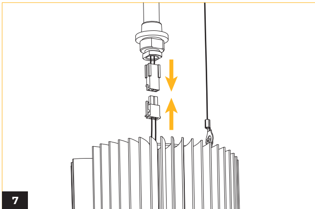
7 Connect the electrical connections.
