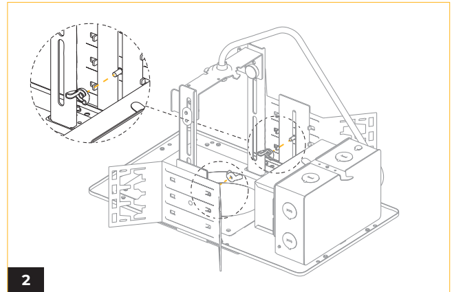
2 Secure the butterfly bracket by screwing in the provided wing nut.
