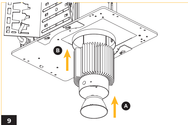
9 Install the reflector on the LED holder in the light engine. Bring the light engine back into the bracket.
