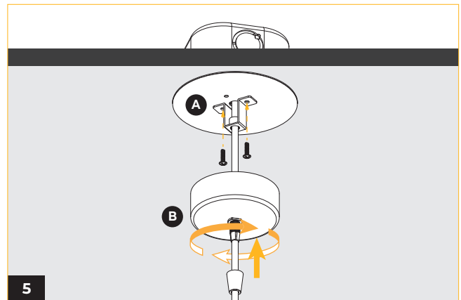
(A) Fasten canopy plate in place using 2 phillips screws. (B) Cover the canopy plate with the canopy cover, and secure it by screwing in the cord grip base.
