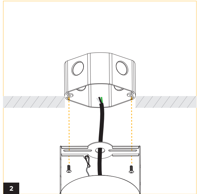
Feed the cord through the hole of bracket and the center hole of cover. Make electrical connections inside junction box (by others). See wiring diagrams.
